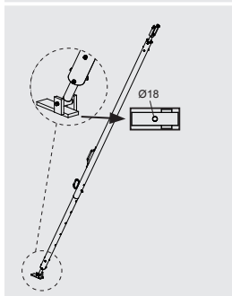
Richtstrebe K440 Aligning strut K440
