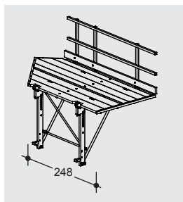
Eck-Klappgerüst L Corner folding scaffold L
