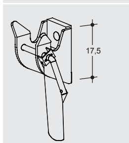
Konsollager Bracket bearing
